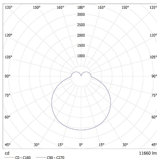
Lucis IR.L12.700M.1 IZAR R MAX LED / LDC (Polar)
